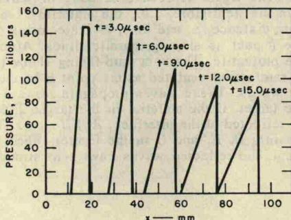
Fig. 3. Profiles of Pressure Behind Shock at Fixed Times (From Fowles)
